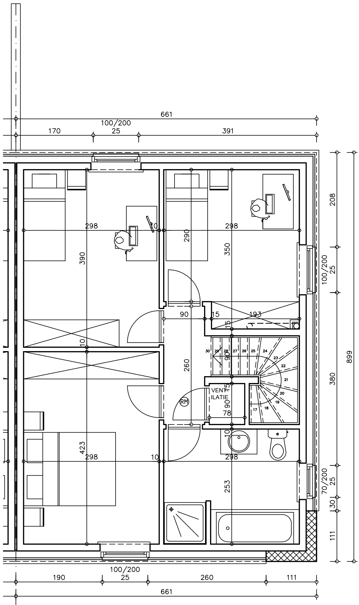
LOT 01 ZOLDER
