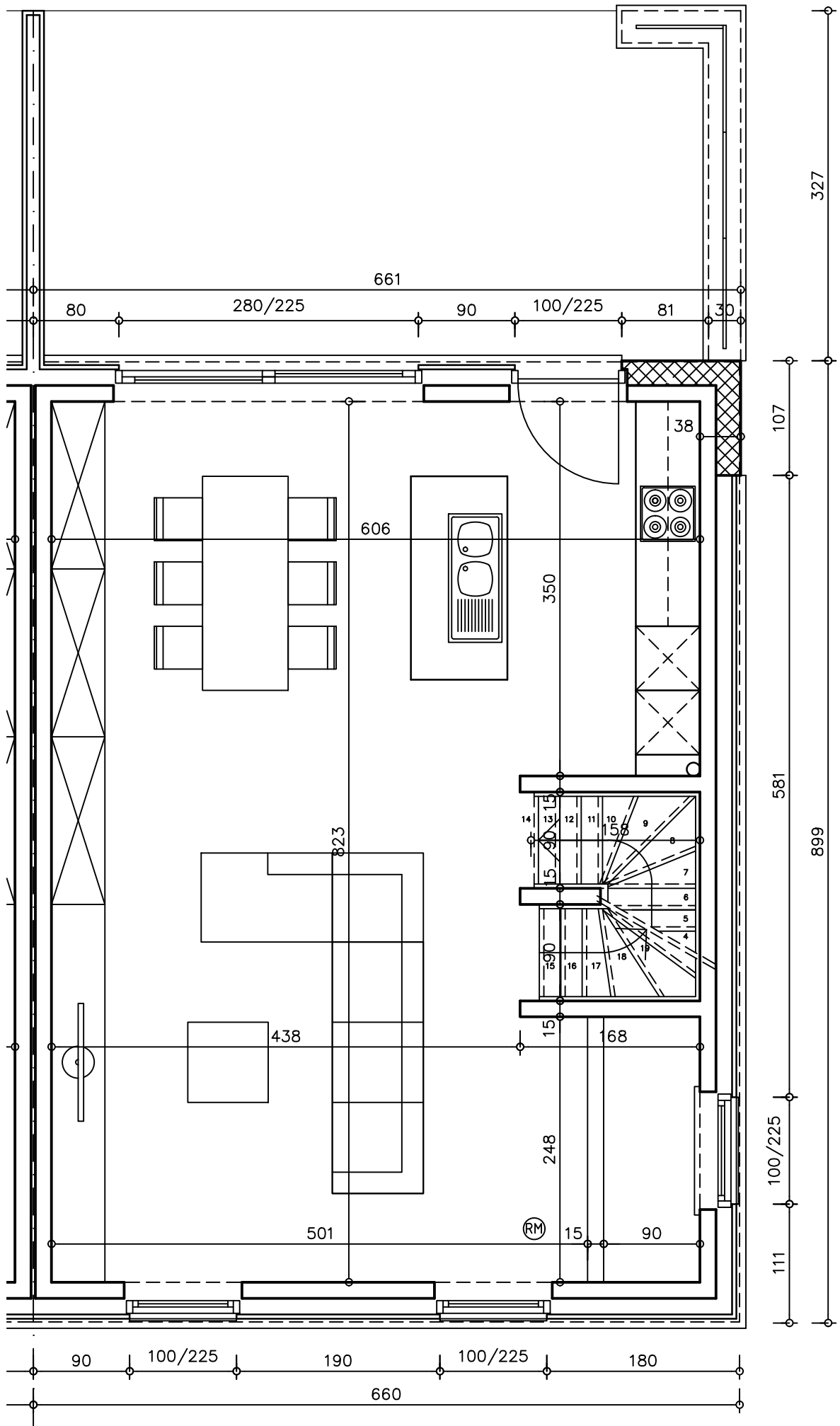
LOT 01 VERDIEPING
